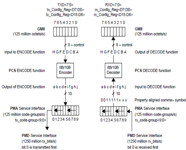
Figure 3. PCS reference diagram
