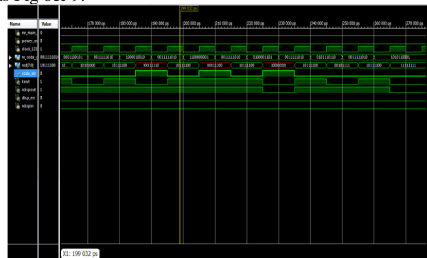
Figure8--8B/10B decoder.
