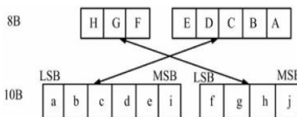
Figure 1. 8B/10B encoding relationship
