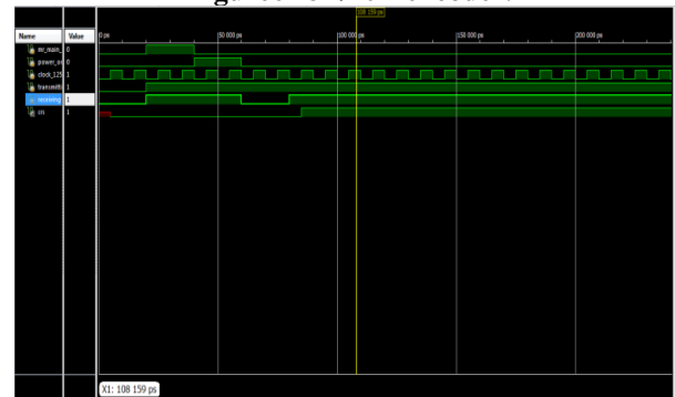
Figure7—Carrier sense.
