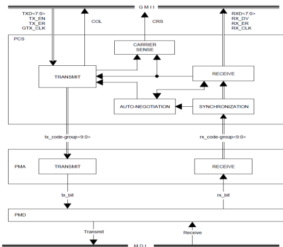
Figure 2. PCS Block Diagram
