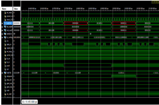
Figure10—final output waveform for PCS in Xilinx.
