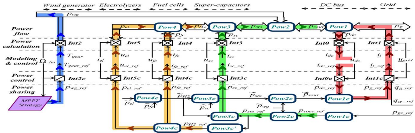
Fig. 6. Multilevel representation of the grid-following strategy
