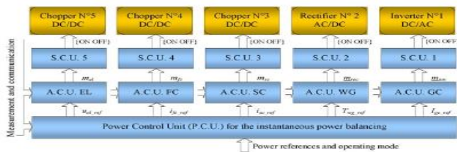
Fig.3.Hierarchical control structure of the HPS
