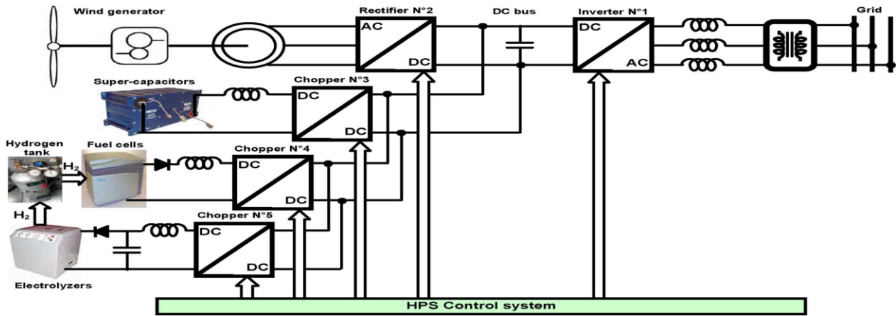
Fig. 2. Structure of the studied wind/hydrogen/SC HPS.
