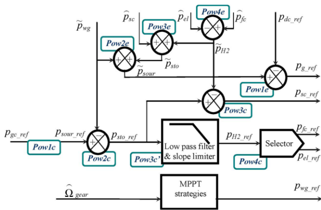
Fig. 7. Block diagram of the grid-following strategy.
