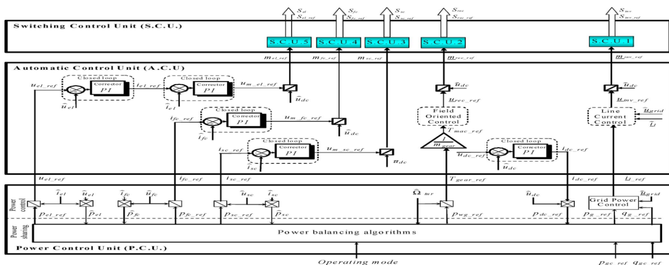
Fig. 4. Modeling and control of the HPS by the Energetic Macroscopic Representation
