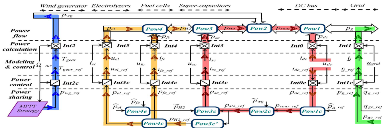
Fig. 8. Multilevel representation of the source-following strategy.
