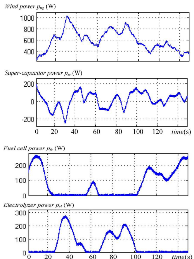
Fig. 11. Power profiles of the different sources.
