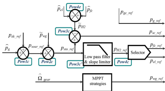
Fig. 9. Block diagram of the source-following strategy
