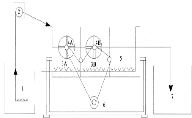
Figure-1. Schematic Diagram of Experimental Setup (RBC-105 L Capacity)
