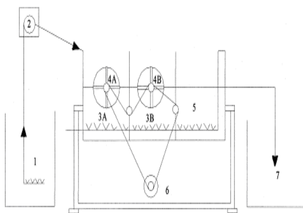
Figure-1. Schematic Diagram of Experimental Setup (RBC-105 L Capacity)
