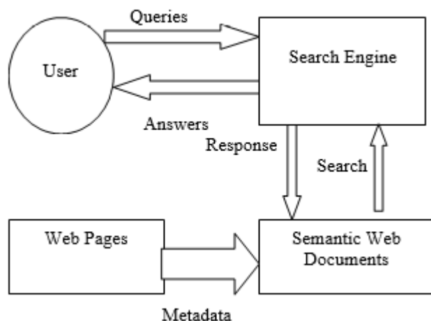
Figure 2. Design Architecture of Intelligent Semantic Web Search Engines
