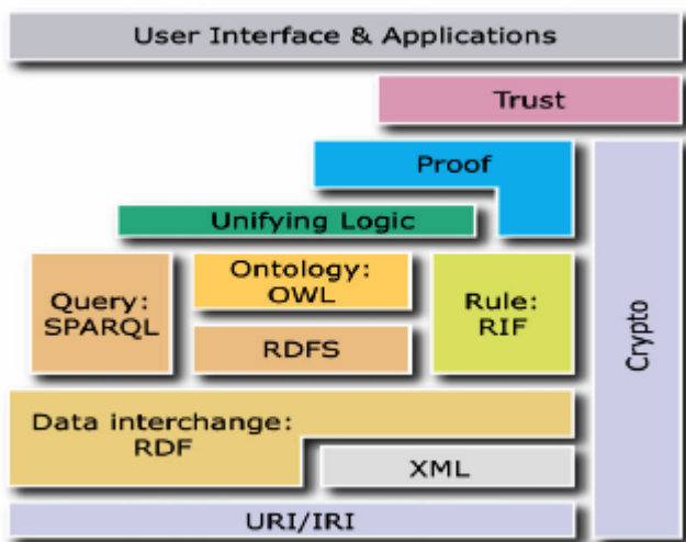
Figure 1: Semantic Web Frame Work
