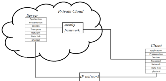
Fig. 6.1 Framework Design
