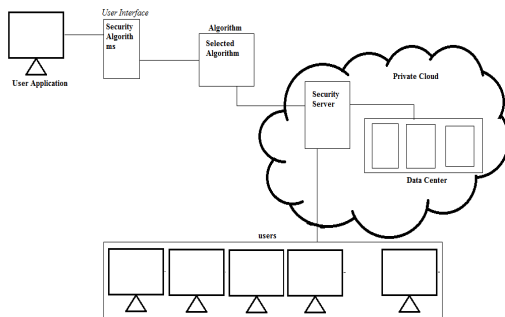
Fig 7.1: System Architecture
