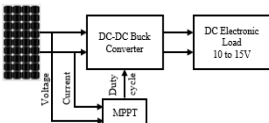
Fig. 2: Use of a buck converter driven by a MPPT control
