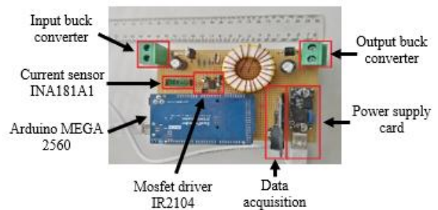
Fig. 6: Prototype used grouping the control and power part
