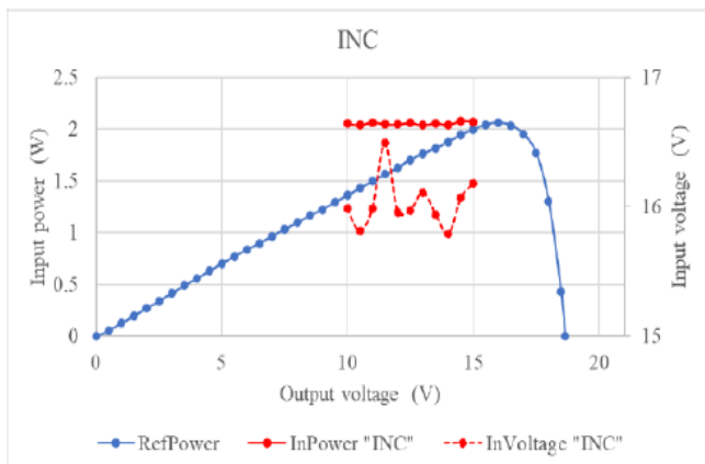
Fig. 15: Input power and voltage with INC
