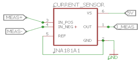
Fig. 5: Current sensor INA181A1
