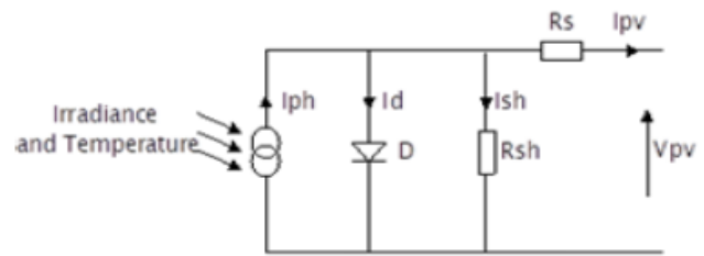
Fig. 3: Single-diode model of a photovoltaic cell
