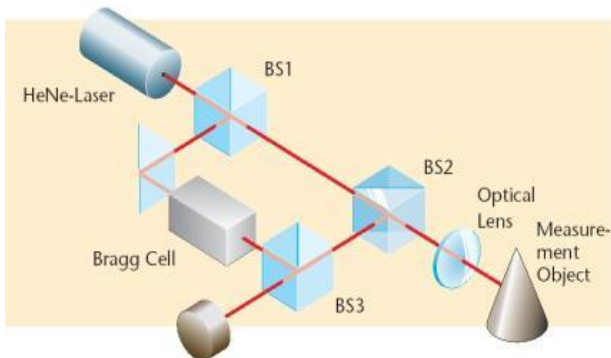
Figure 5. Beam Deflection Method for LDV Sensor [36]
