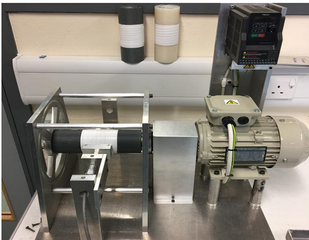
Figure 9. Test Rig used to conduct the experiment [49]
