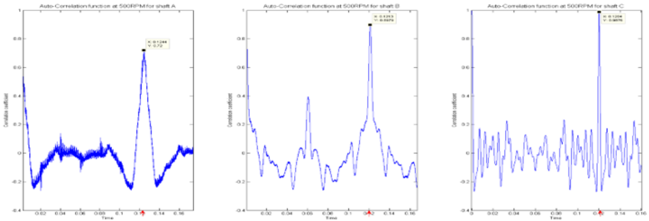
Figure 14. Autocorrelation Function for shaft A to C at 500 RPM
