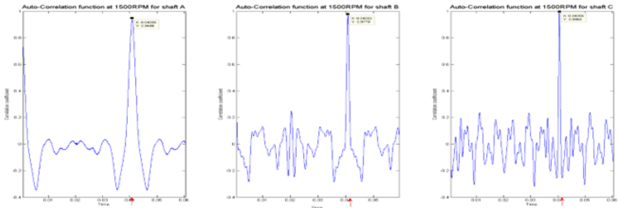
Figure 15. Autocorrelation Function for shaft A to C at 1500 RPM
