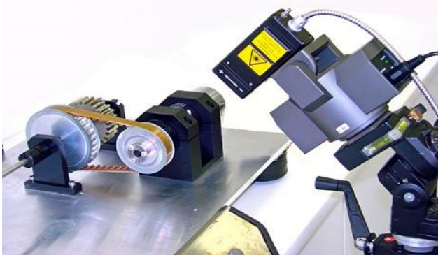
Figure 6. Photo of LDV Sensor [37]
